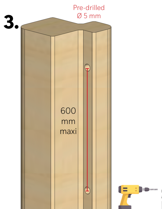
Profile on inside corner
