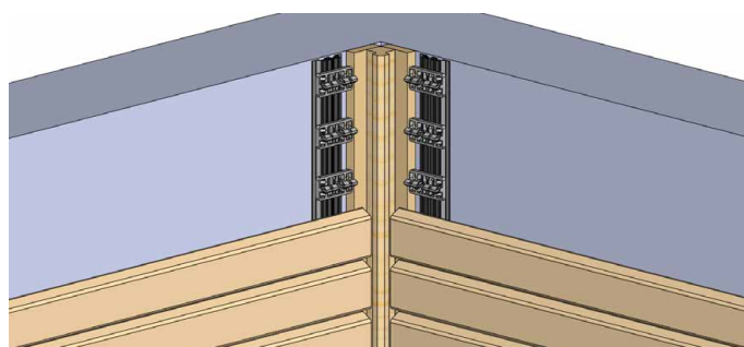
Profile on inside corner
